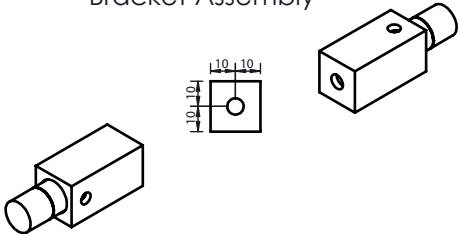
Bracket Assembly
