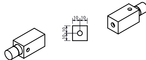
Bracket Assembly
