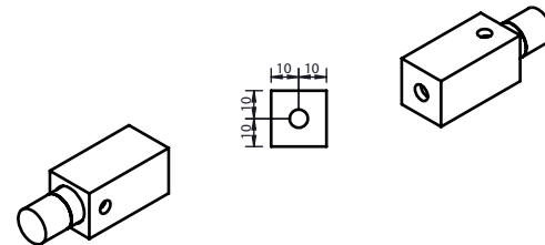
Bracket Assembly
