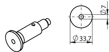
Bracket Assembly
